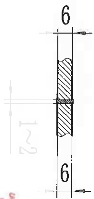
BACK RING WELDING DETAIL 衬圈焊接详图 NO SCALE
